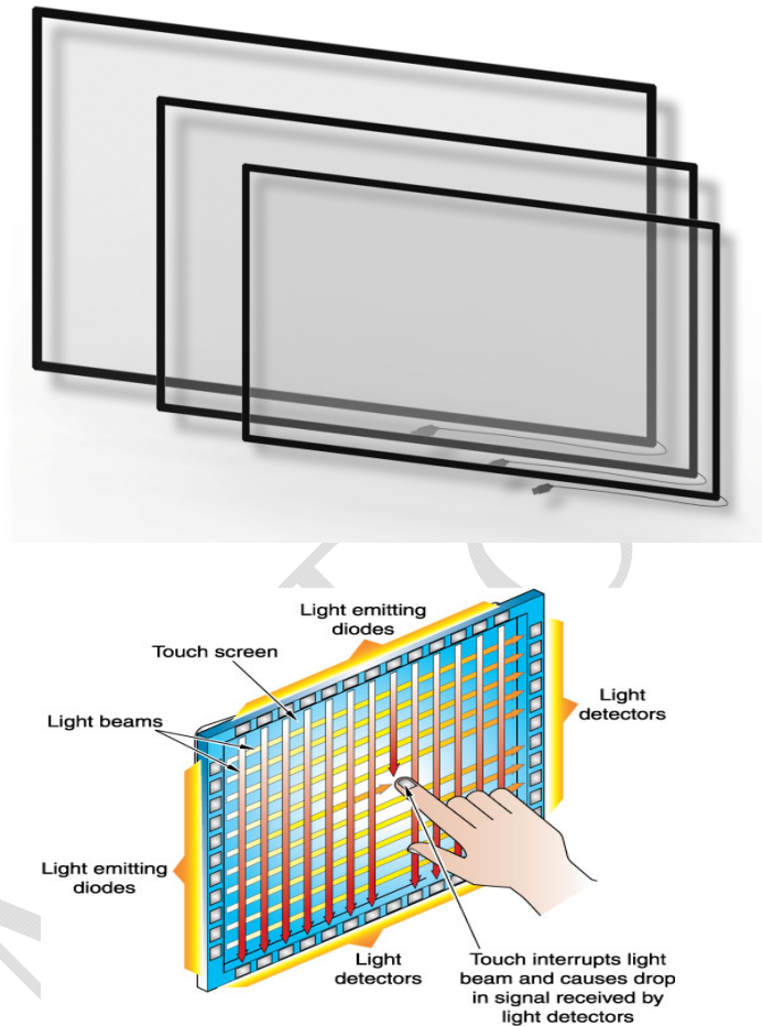
Fig. 1 The principle of infrared touch screen
