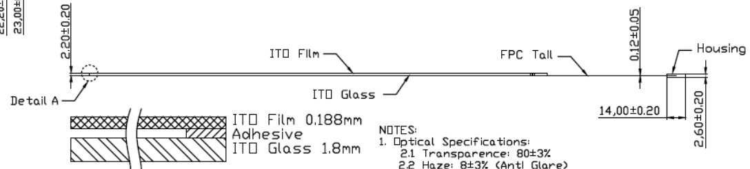
Detail A
