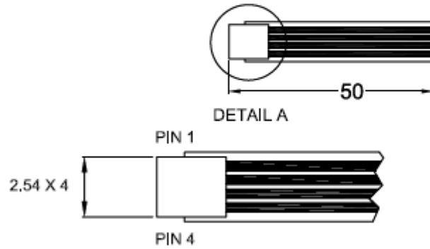
DETAIL A
